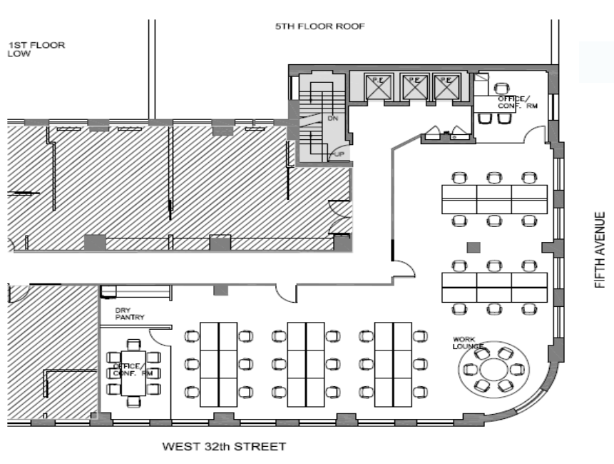
601 – 605 – 3,616 RSF - Office Test Fit – Open Plan
